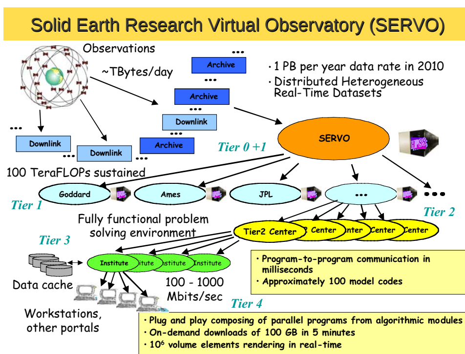
Figure 1. Solid Earth Research Virtual Observatory (SERVO) and associated computational framework for supporting solid Earth science missions, data, analysis, and modeling.
