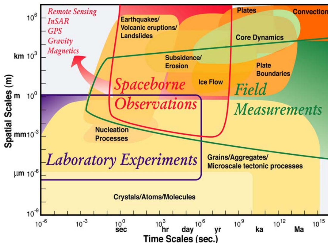
Figure 2. The physical processes associated with the solid Earth take place on many scales of space and time. Simulations and theory must account for how these many scales interact.
