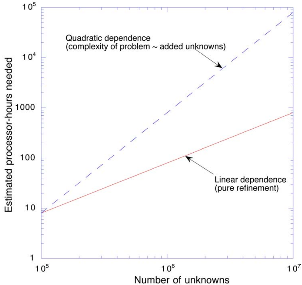
Figure 3. Processor time increases linearly with mesh refinement. Adding complexity increases the unknowns and solution time is quadratic in unknowns.
