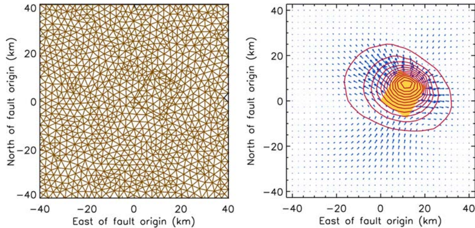
Figure 4. A Northridge class simulation with 100,000 unknowns, and 4000 time steps takes 8 hours on a high-end workstation. Modeling the southern California system requires 4 million unknowns thus taking 12,800 processor hours for 1 km resolution. 0.5 km resolution would take 100,000 processor hours or 400 hours (17 days) on a dedicated 256-processor machine.
