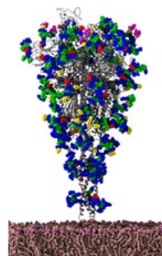
SARS-CoV-2 spike protein of the corona virus, as simulated at an academic lab using NSF’s Frontera supercomputer, in work funded by NIH and NSF. Source: NSF Fact Sheet 4-10-20.
